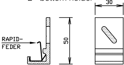
L 2 bottom holder
