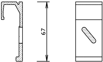
L 2 top holder
