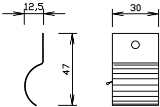
FEDER (spring)
