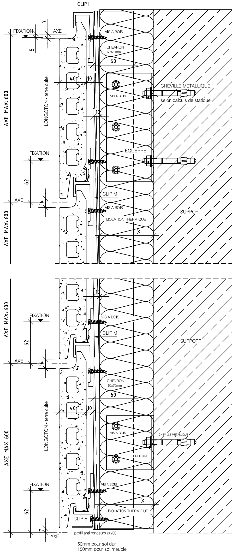
LONGOTON® - QF Coupe verticale Figure 11
