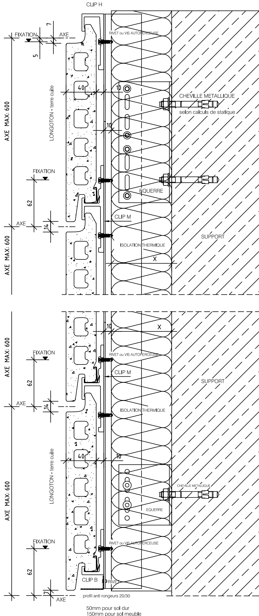
LONGOTON® - QF Coupe verticale Figure 11.1
