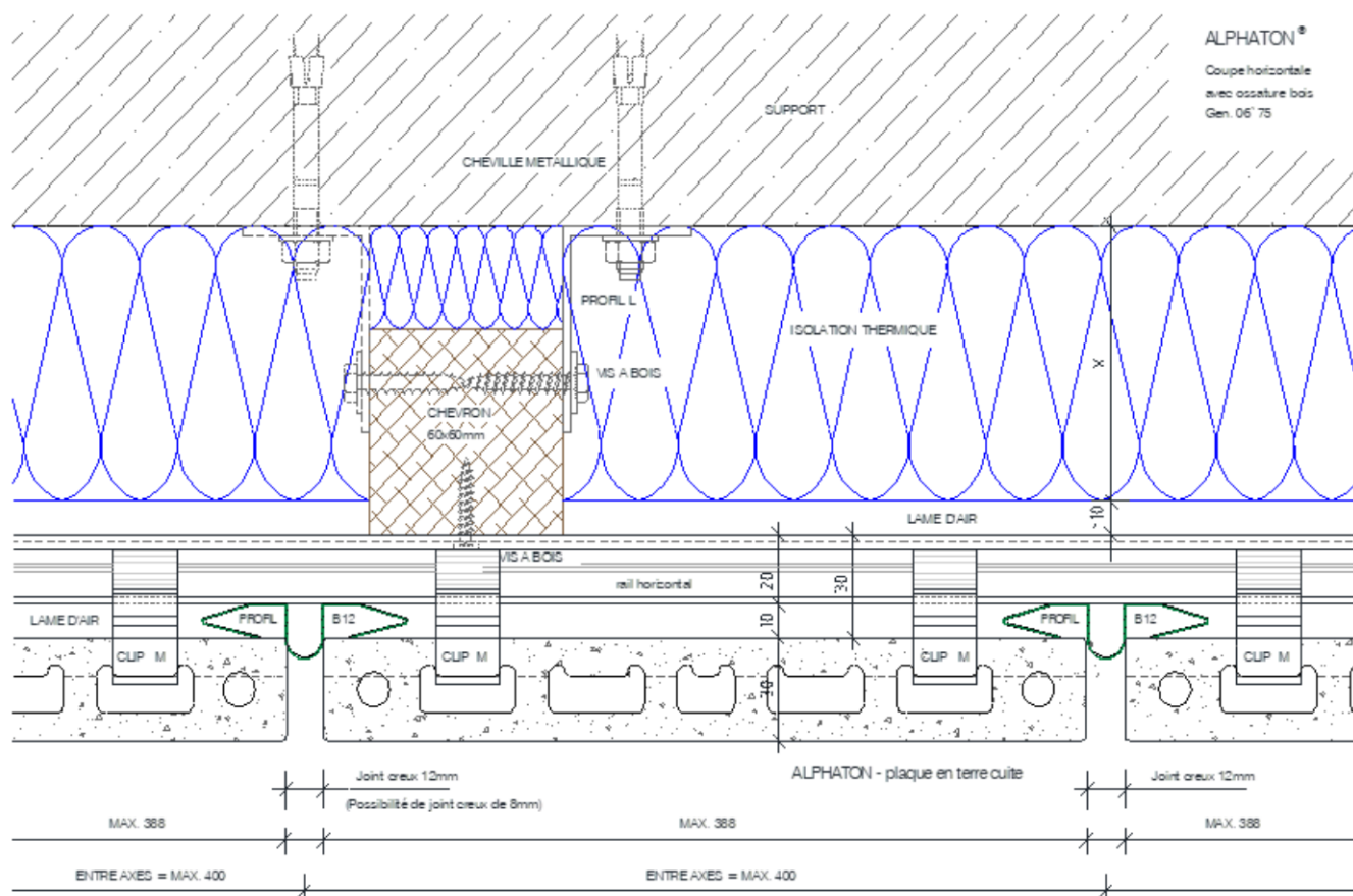
Figure 30 - Coupe horizontale
