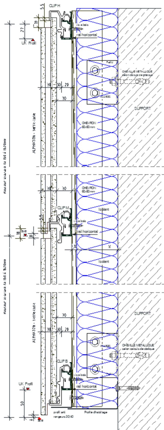
Figure 32 - Coupe verticale
