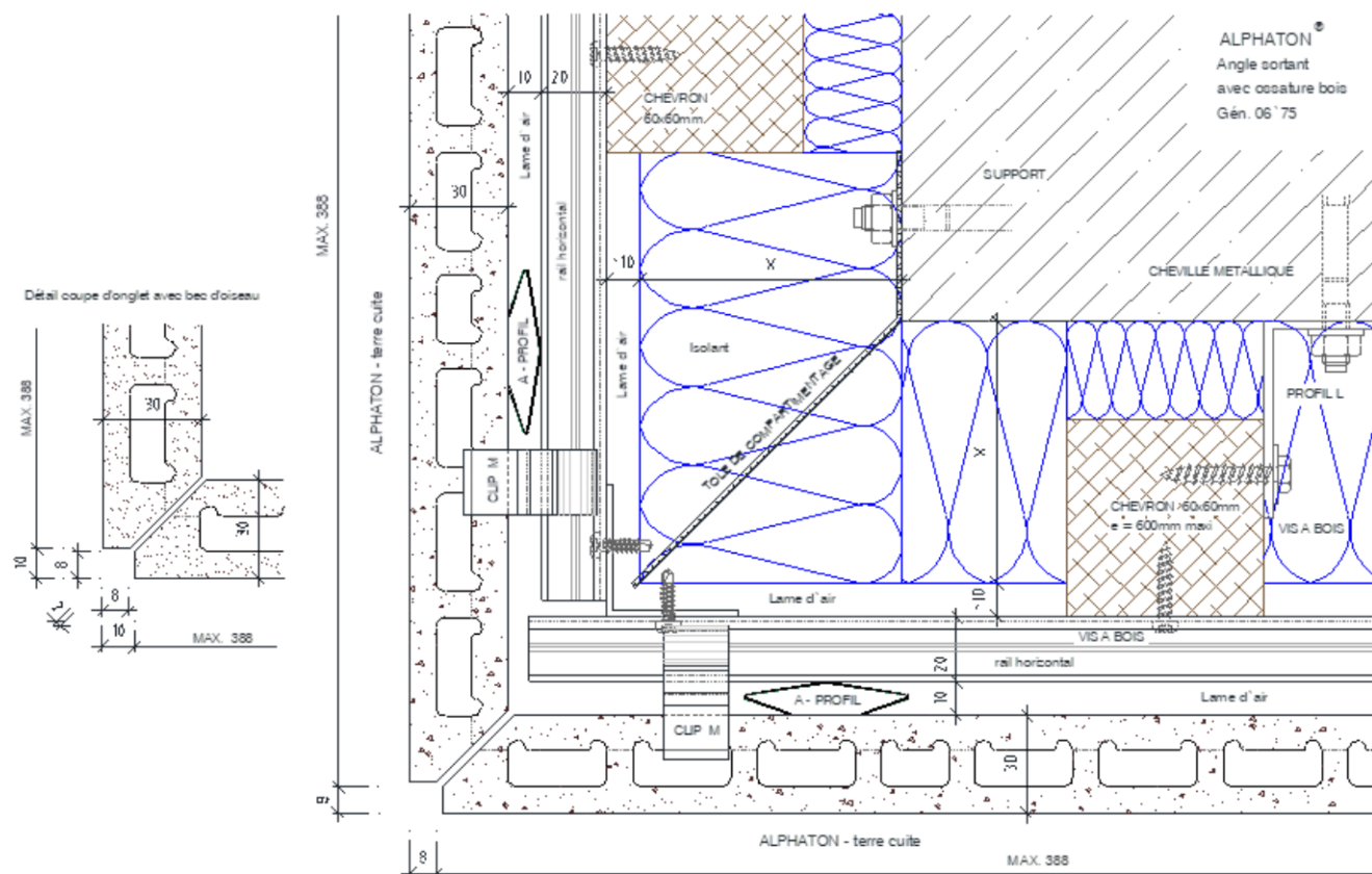
Figure 35 - Angle sortant
