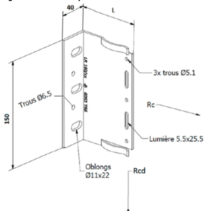
Figure B2 – Pattes-équerres ISOLALU+ LR160x200x50mm
