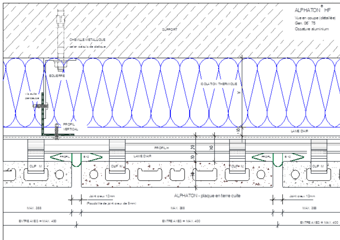
Figure 11 - Coupe horizontale
