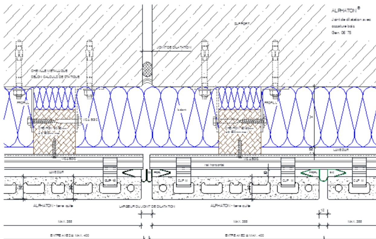
Figure 39 – Joint de dilatation
