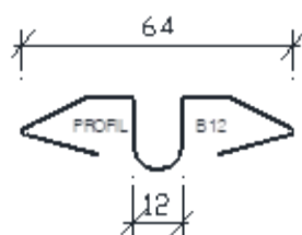
Figure 4 - Profils de joint ressort vertical
