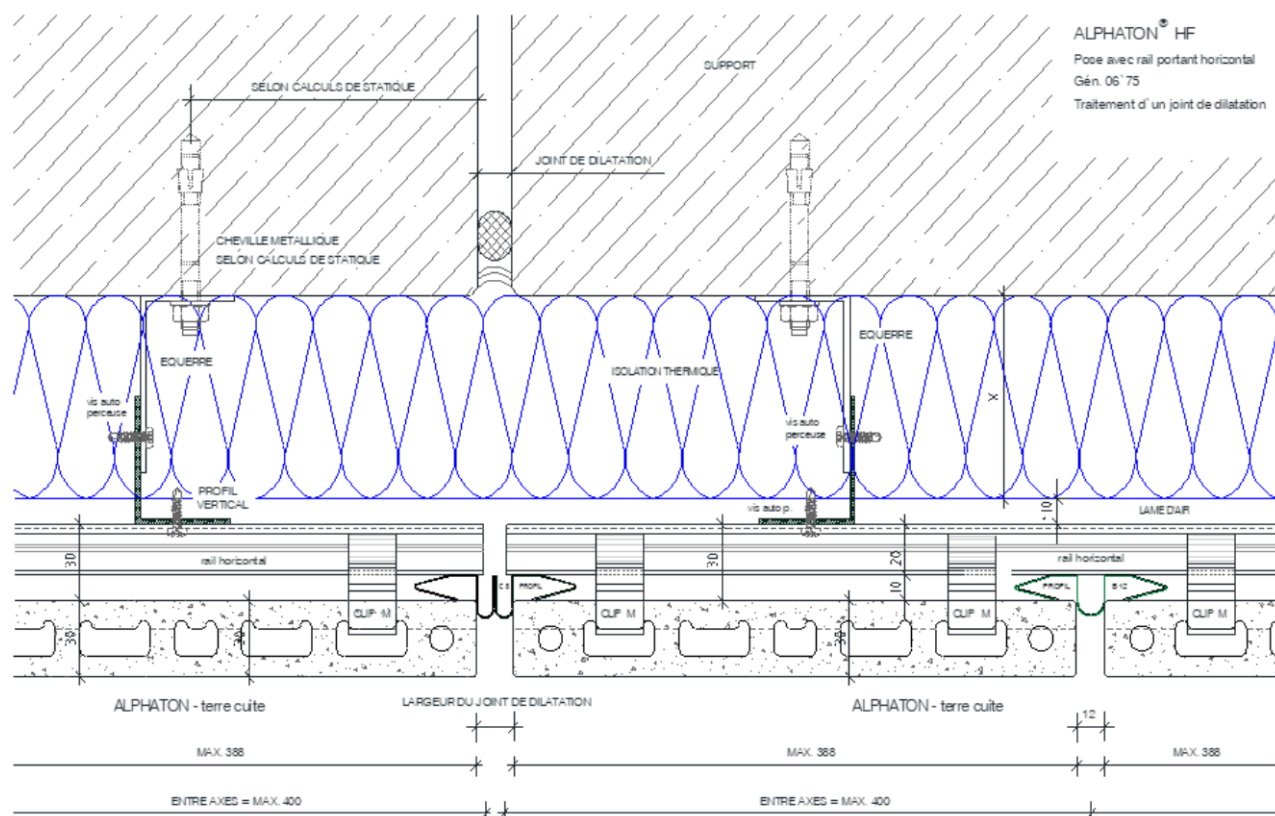
Figure 28 - Joint de dilatation
