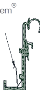
Figure 4 - Profils de joint ressort vertical
