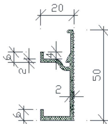
Figure 6 - Rail portant horizontal 06'75
